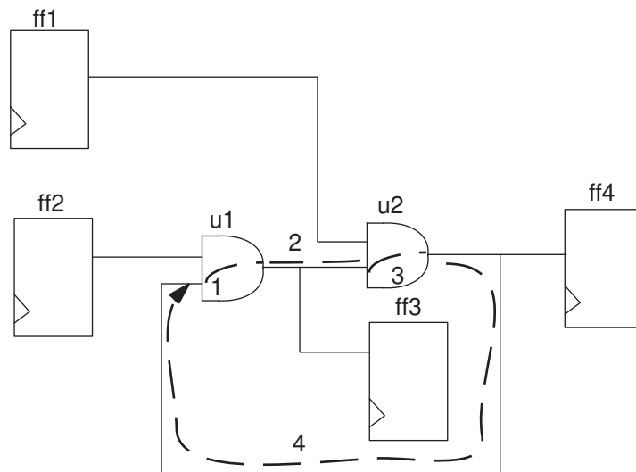
Figure 203 Loop breaking example
