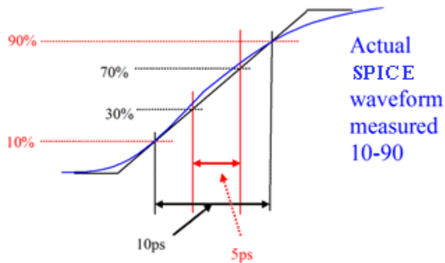
Figure 30 SPICE waveform
