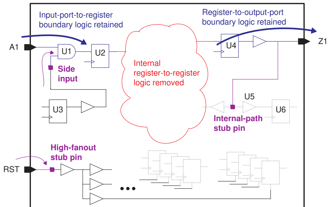
Figure 384 HyperScale Block Model
