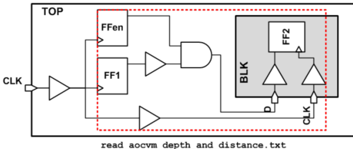
Figure 421 AOCV modeling
