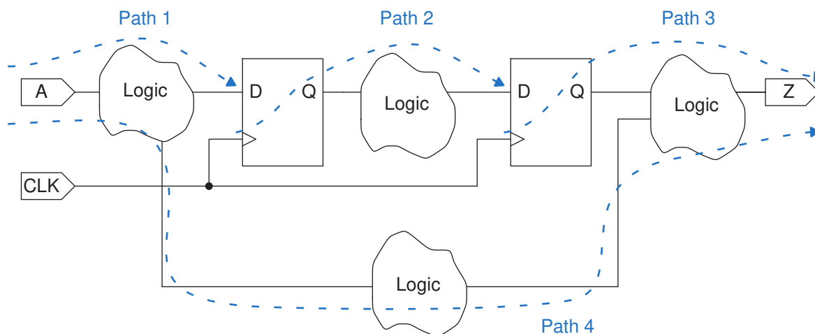
Figure 2 Timing paths
