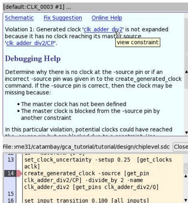
Figure 286 Definition of clk_adder_div2 Generated Clock in Constraint File
