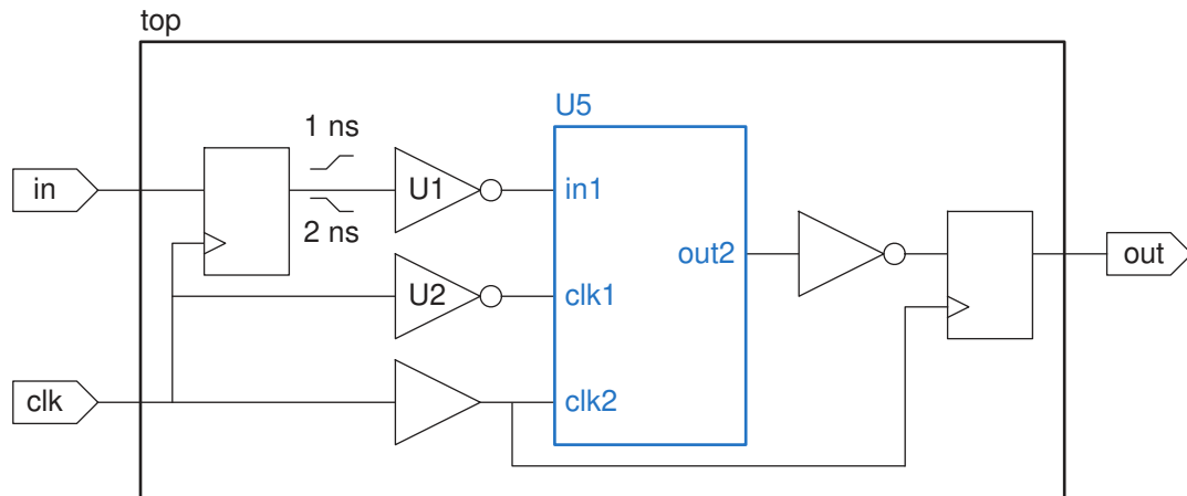
Figure 423 Context characterization example
