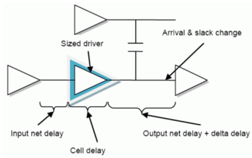
Figure 378 Parameters Considered by ECO Timing Estimation
