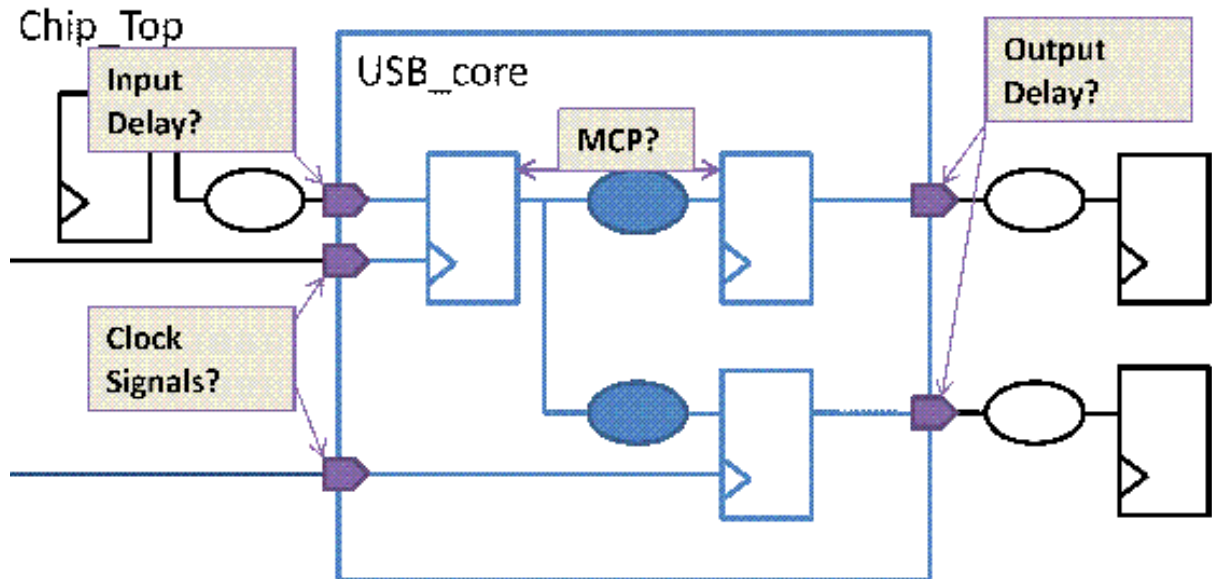
Figure 251 Block Design USB_core Inside Design Chip_Top
