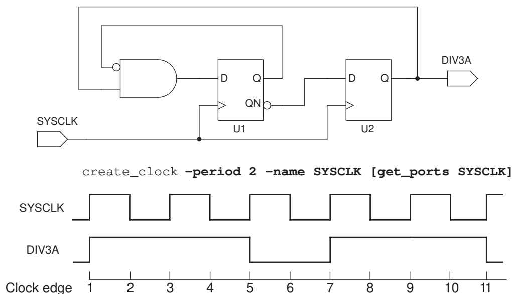
Divide-by-3 clock generator
