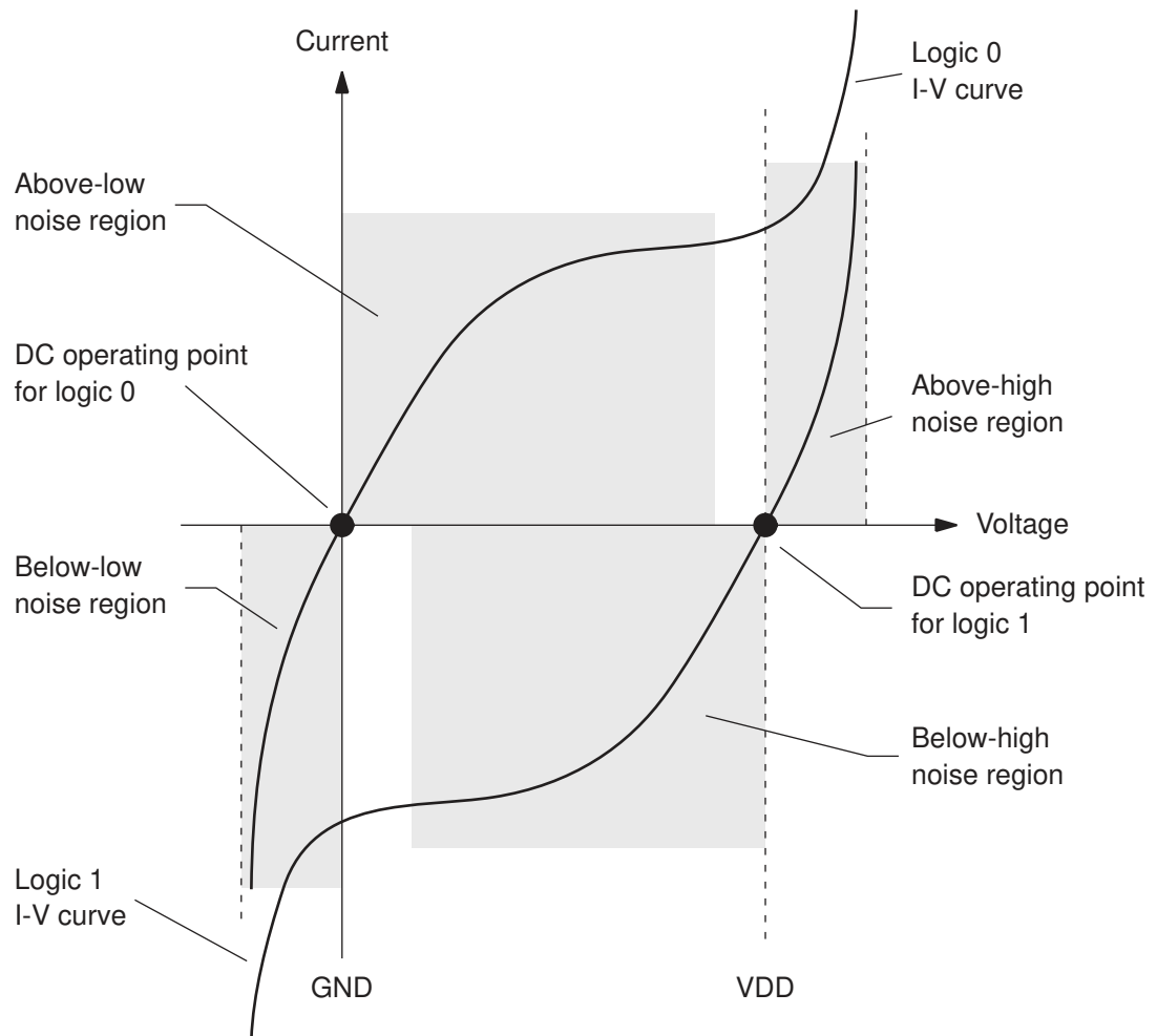
Figure 190 Steady-state I-V characteristics at a CMOS output
