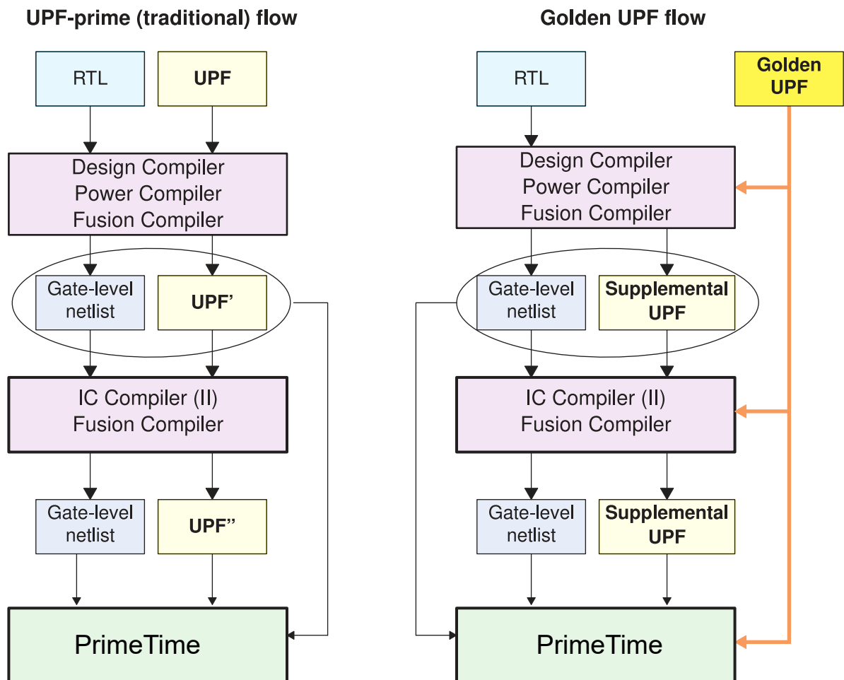
Figure 141 UPF-Prime and Golden UPF Flows
