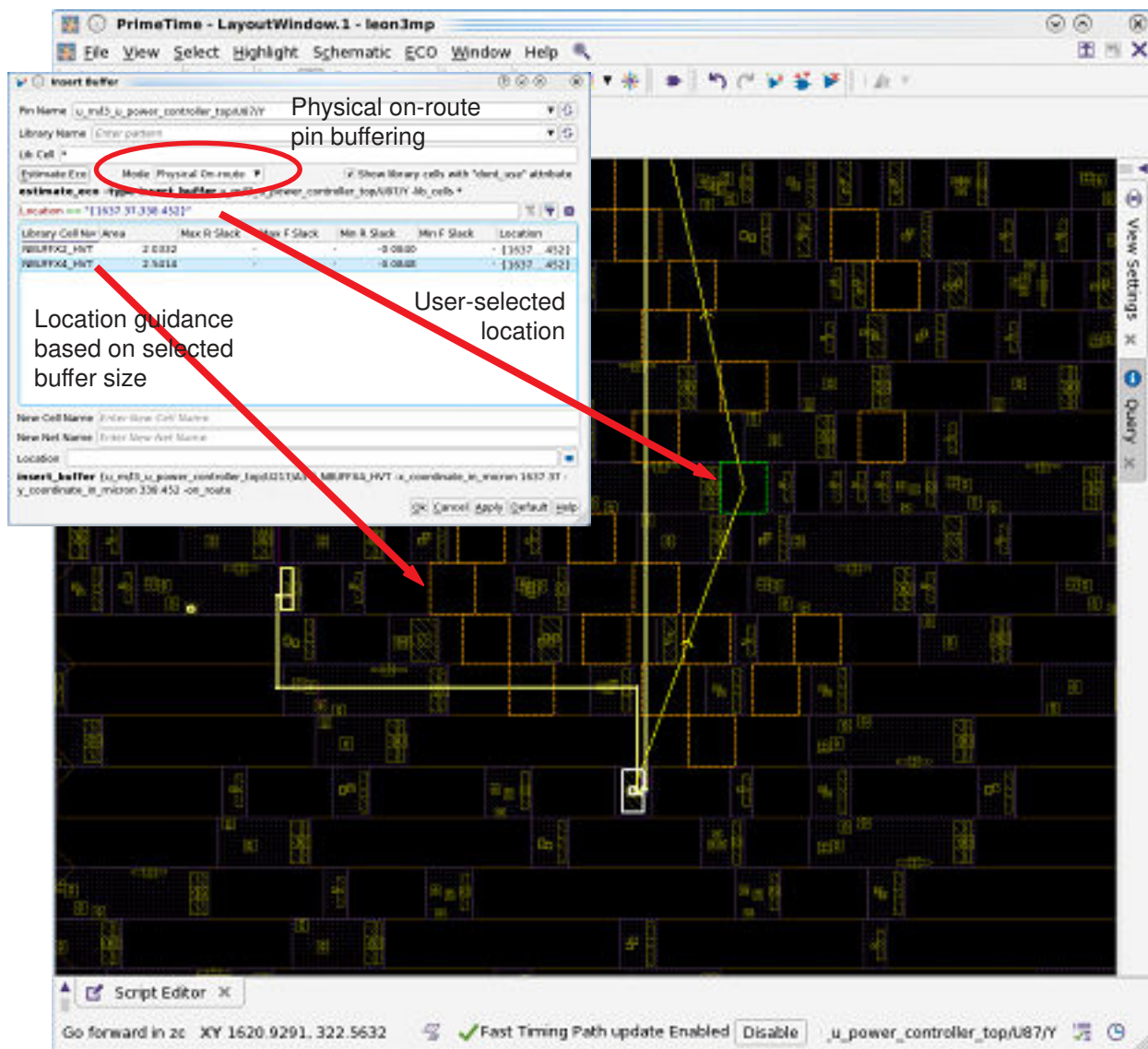
Figure 351 Manual ECO Operations in the GUI
