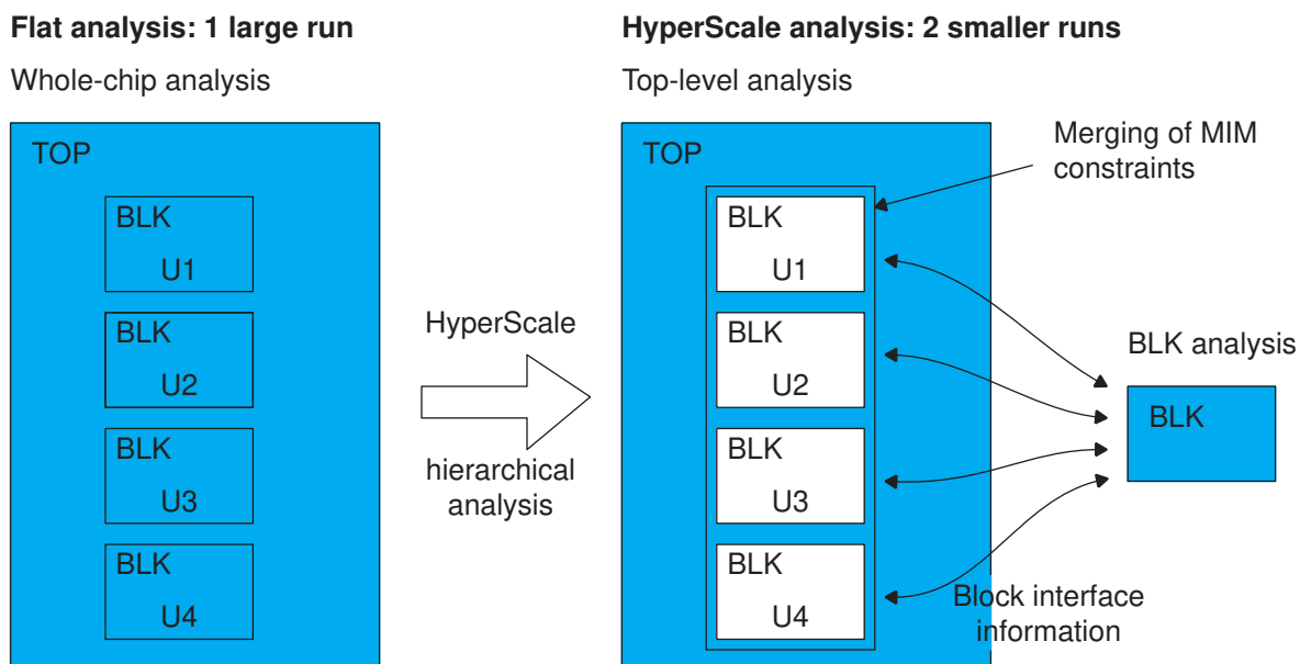
Figure 386 Context Merging for Multiply Instantiated Modules
