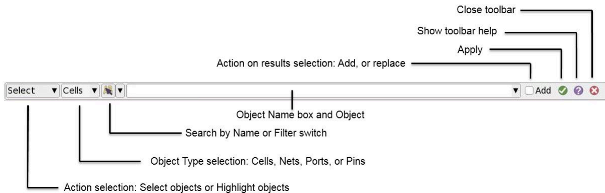
Figure 268 Select By Name Toolbar
