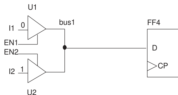
Figure 205 Circuit example
