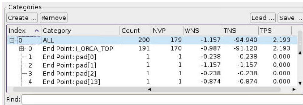
Figure 312 Path List Updated With New Categories
