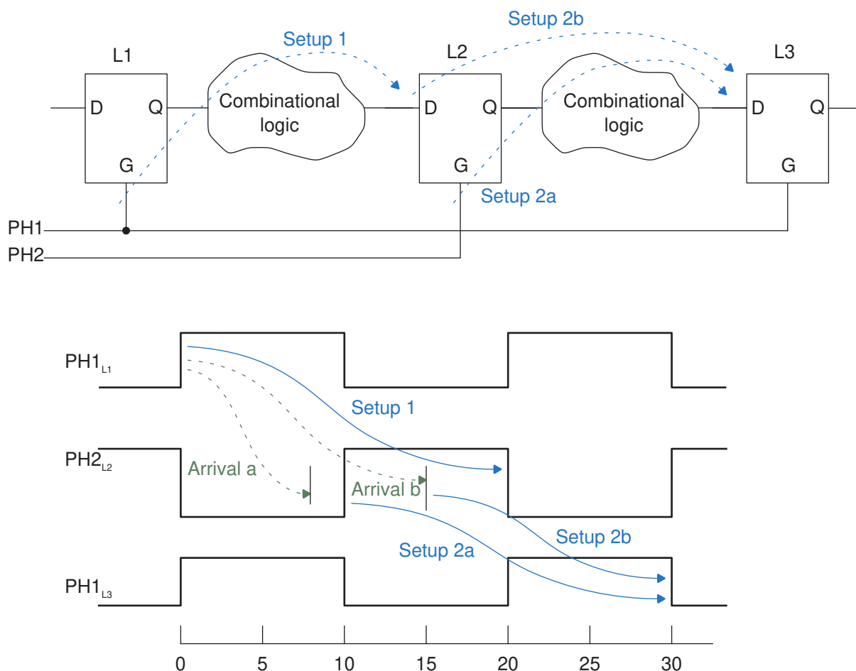
Figure 6 Latch-based paths
