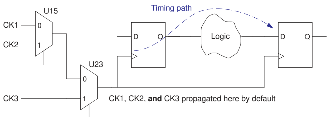
Figure 50 Multiplexed Clocks
