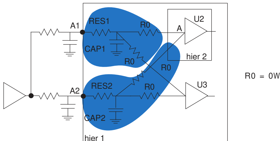
Figure 125 Multidrive segments
