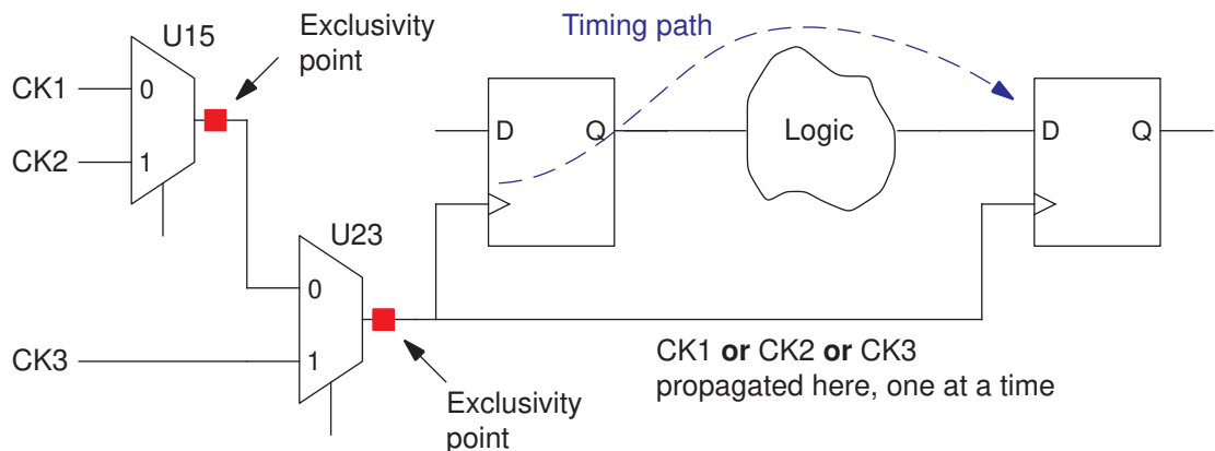
Figure 51 Multiplexed Clocks With Exclusivity Points
