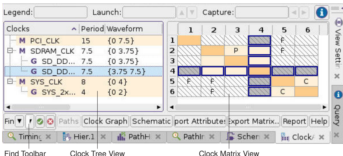
Figure 320 Clock Analyzer
