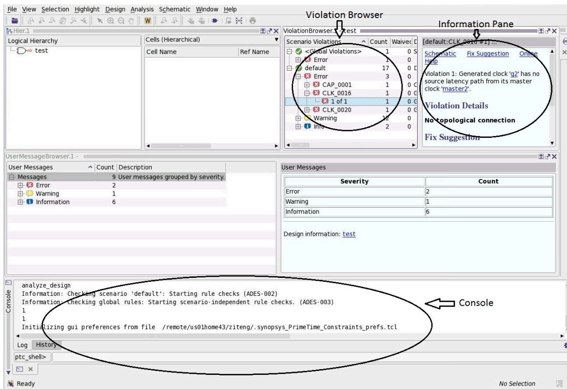
Figure 259 Constraint Consistency Window on Startup
