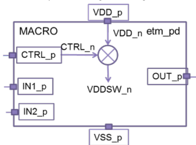
Figure 437 Simple multivoltage test design
