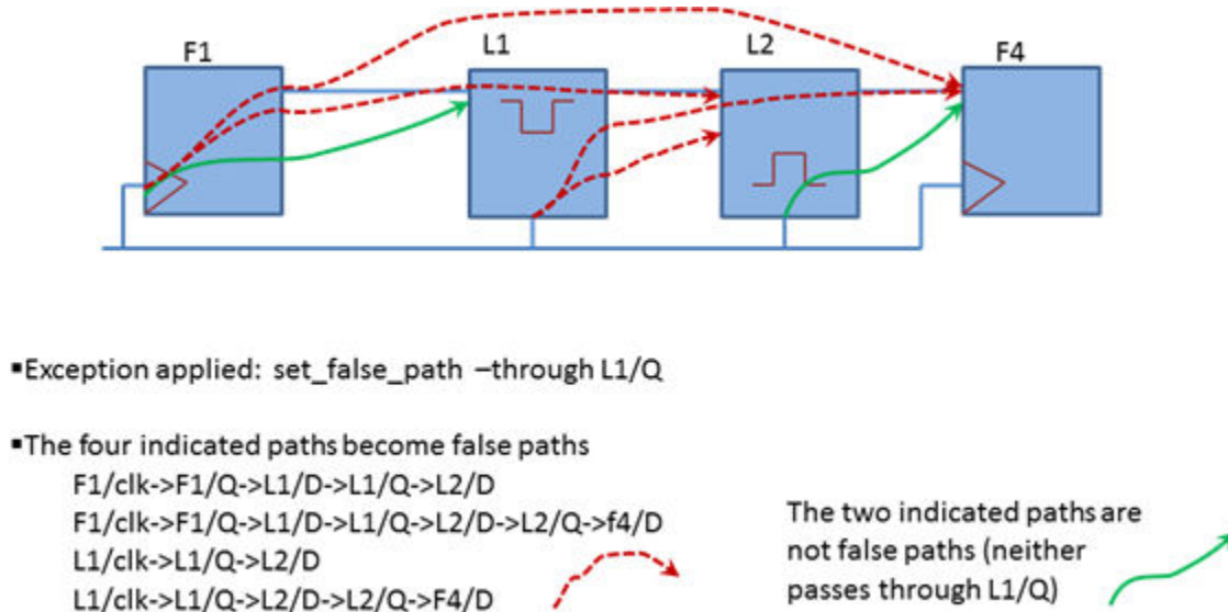
Figure 221 False path exceptions on throughpaths
