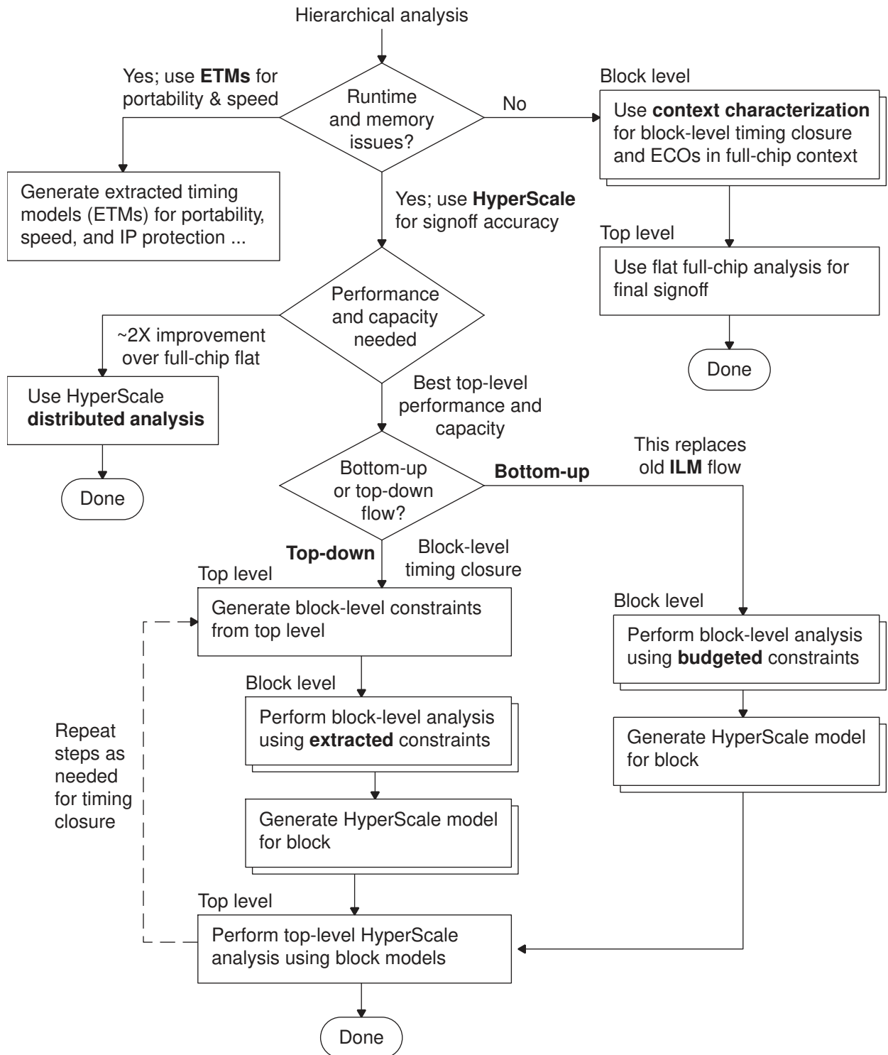
Figure 381 Hierarchical Analysis Flows
