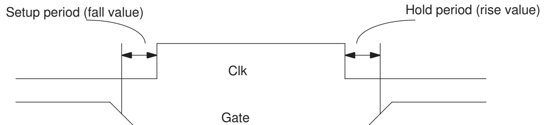
Figure 446 NOCHANGE_LOW_HIGH arc
