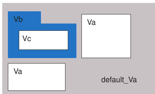
Figure 359 Multivoltage Physical Constraint Example
