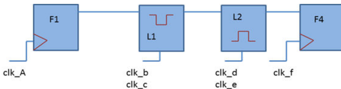
Figure 223 Circuit with multiple clocks at latches
