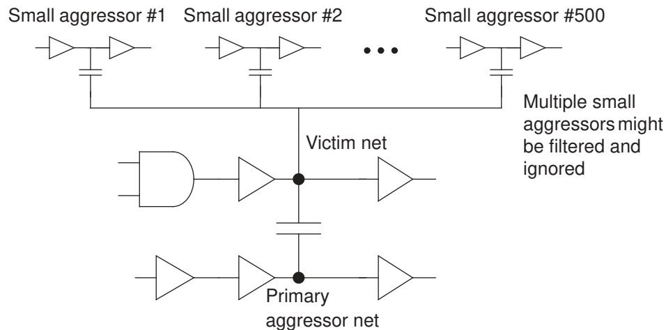
Figure 167 Composite aggressor mode disabled
