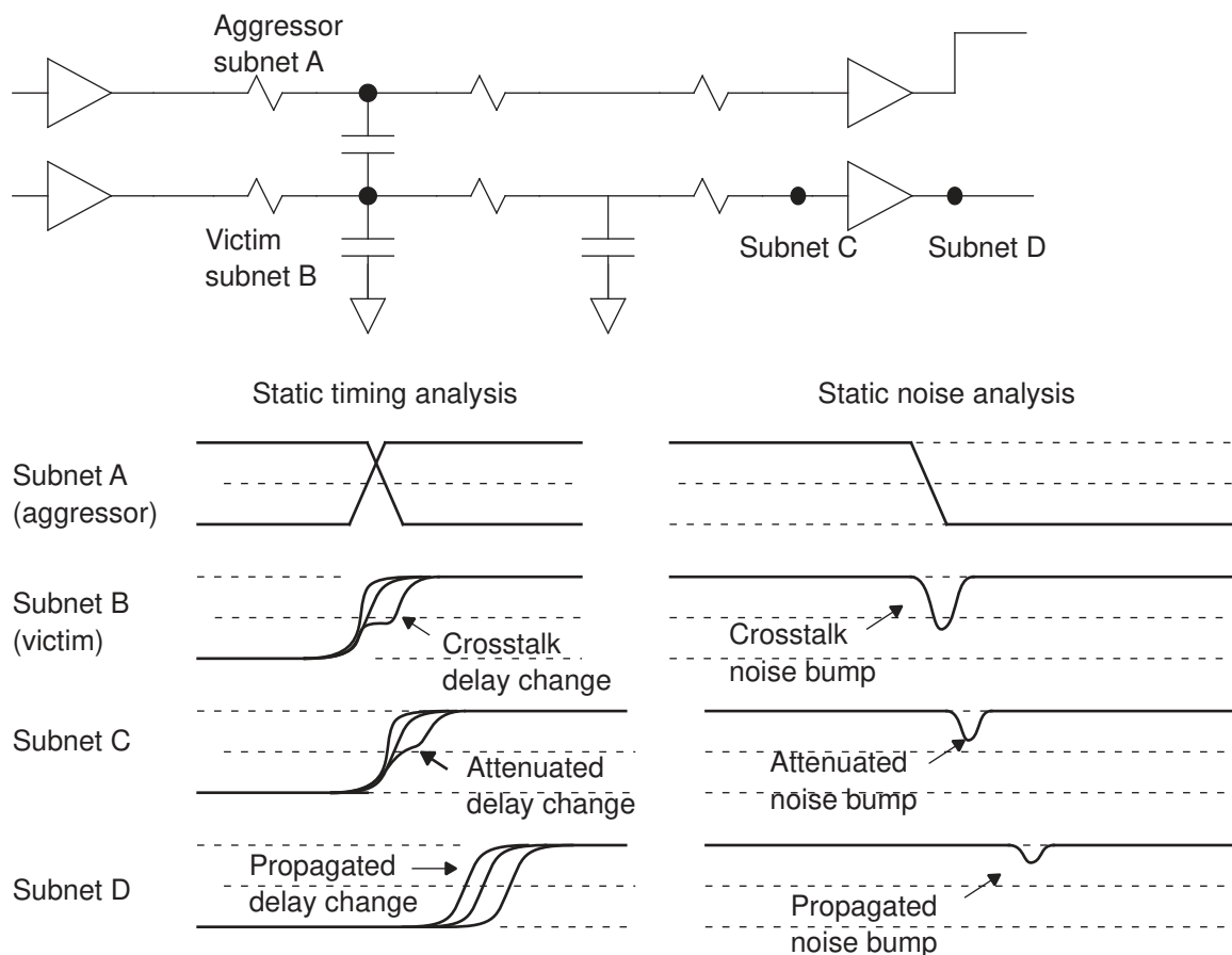
Figure 175 Crosstalk effects on timing and steady-state voltage
