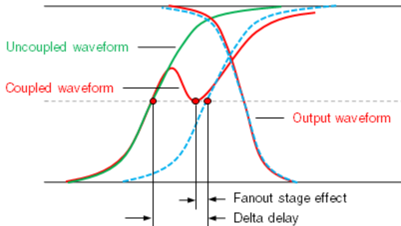
Figure 149 Delta delay includes the fanout stage effect
