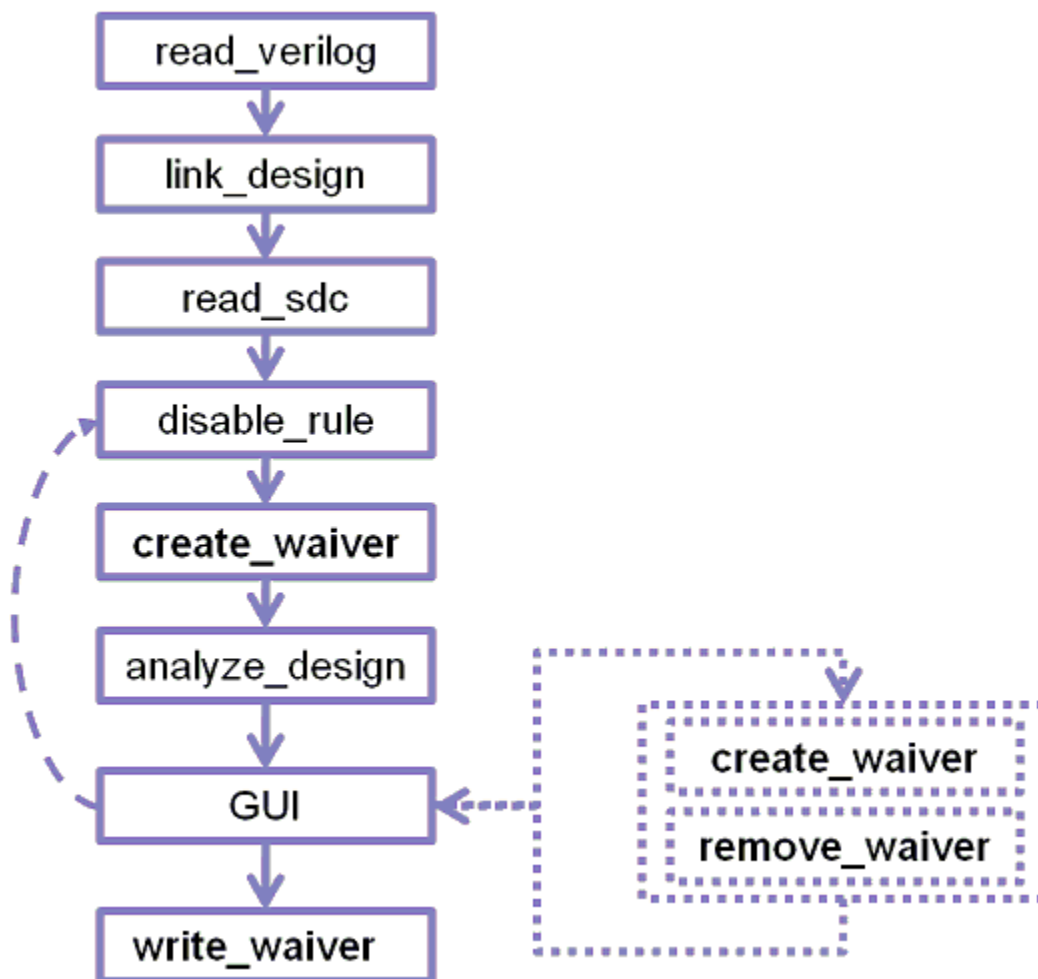
Figure 235 Violation Suppression Usage Model
